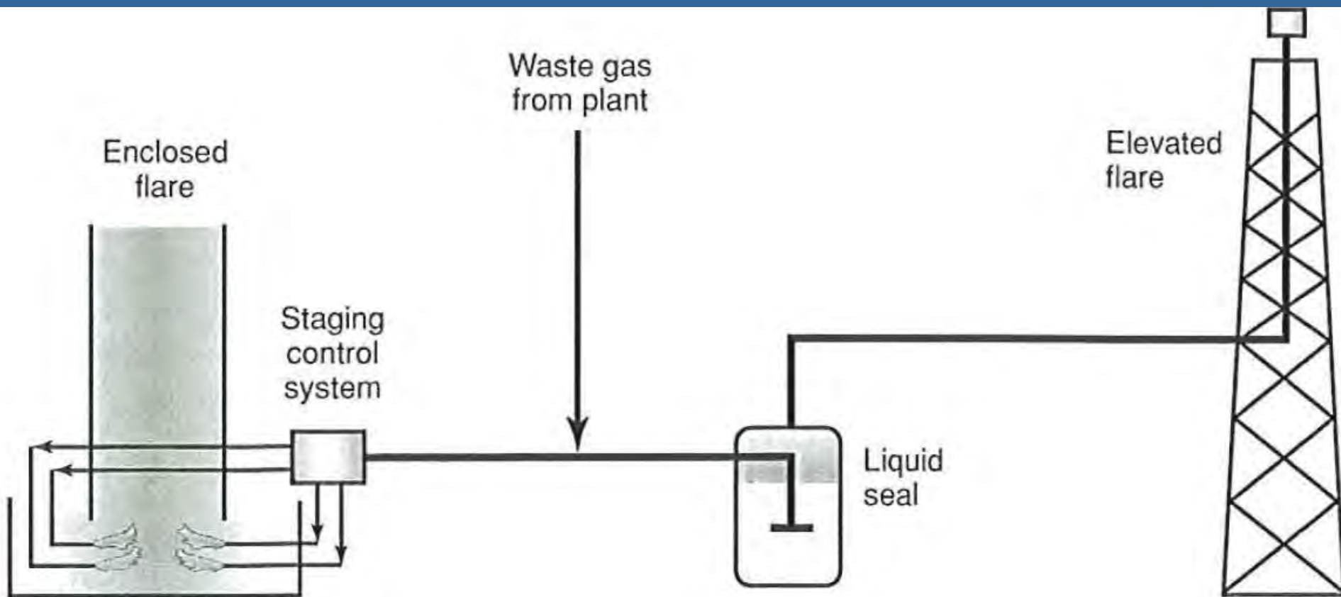
Figure 16—Typical Enclosed Flare Staged to Elevated Flare
