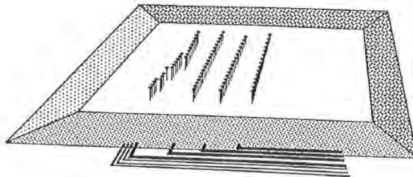
Figure 6—Multi-Burner Staged Flare
