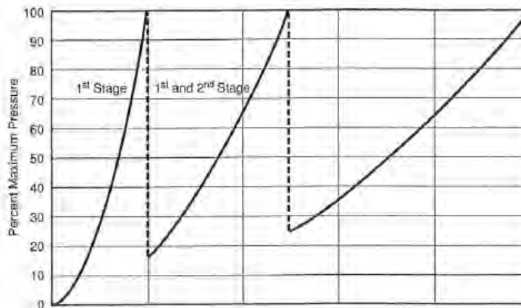
Figure 7—Multi-Burner Flare Staging Curve
