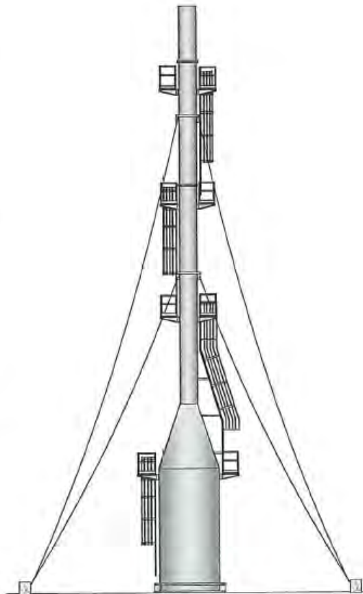
Figure 2—Guyed-Supported Structure
