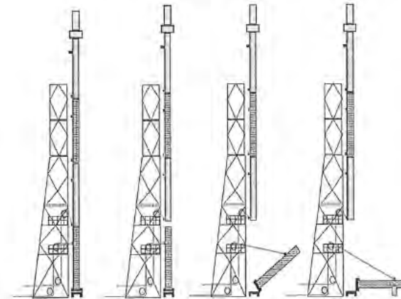
Figure 3b—Demountable Derrick-Multiple Section Riser
