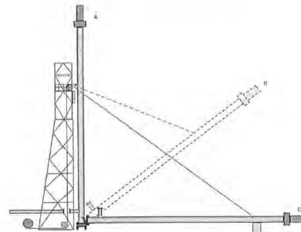
Figure 3c—Demountable Derrick-Single Section Riser
